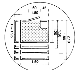
9 Sizes of cold stores (useful area 1.23-3.06 m 2 )
